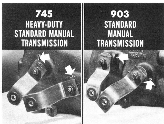
Fig. 16—Retainer pins identify transmission
