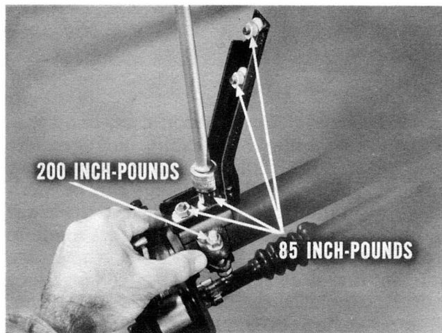
Fig. 5—Steering column jacket centered
