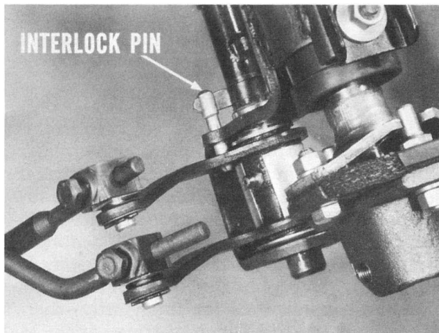
Fig. 1—Heavy-duty linkage
