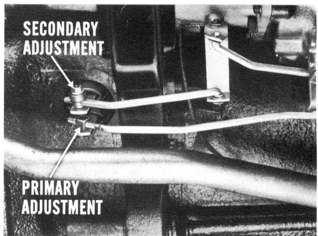
Fig. 14—Control rod adjustment points
