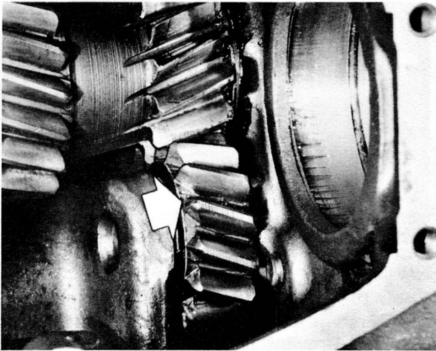
Fig. 19—Reverse idler properly installed
