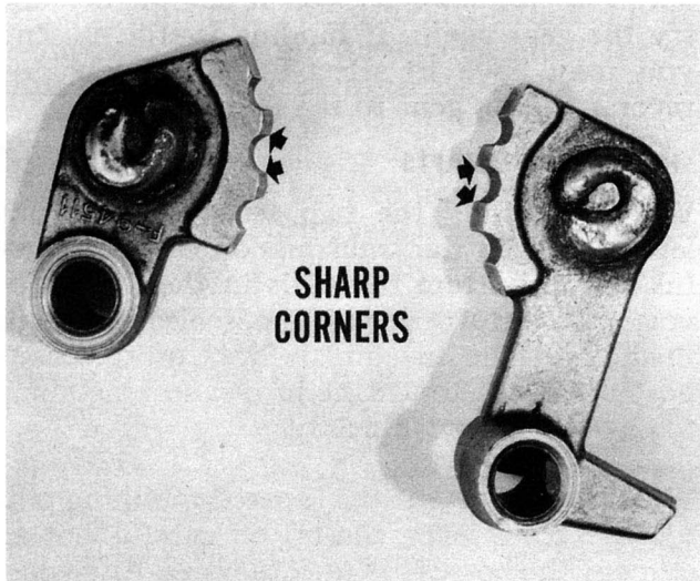
Fig. 17—Stone-off neutral detent notch
