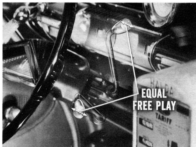
Fig. 6—Test crossover pin travel
