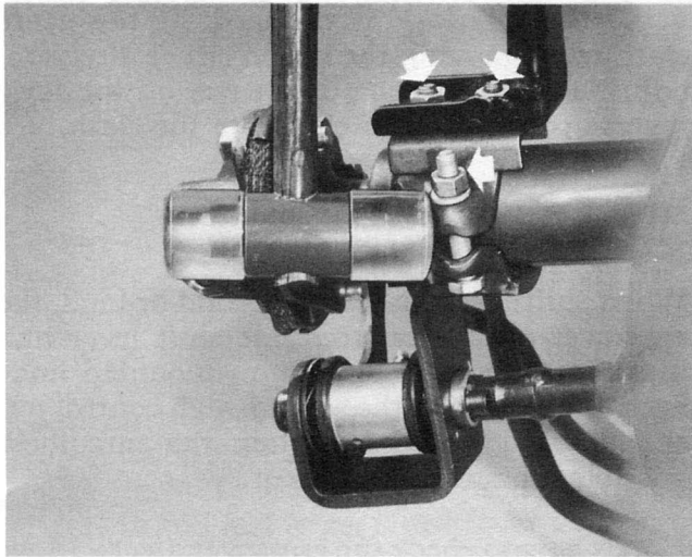
Fig. 7—Adjust crossover pin travel
