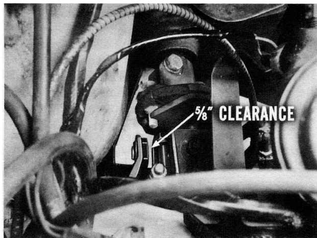
Fig. 4—Shift lever bracket clearance
