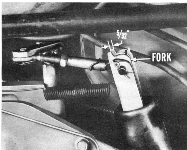
Fig. 15—Clutch free play
