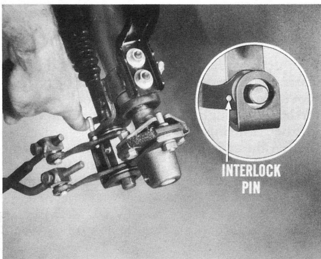
Fig. 10—Center the interlock pin
