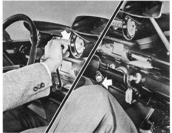
Fig. 8—Adjust gearshift lever position
