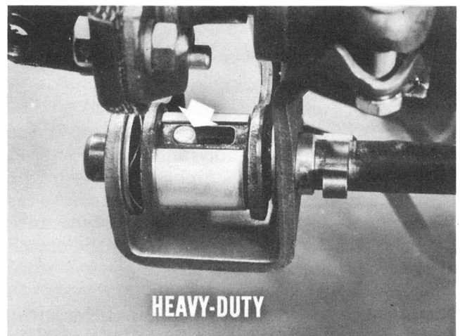
Fig. 3—Crossover pin—heavy-duty linkage
