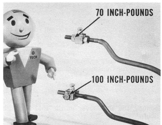
Fig. 9—Swivel types and torques
