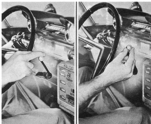
Fig. 11—Test crossover "feel"
