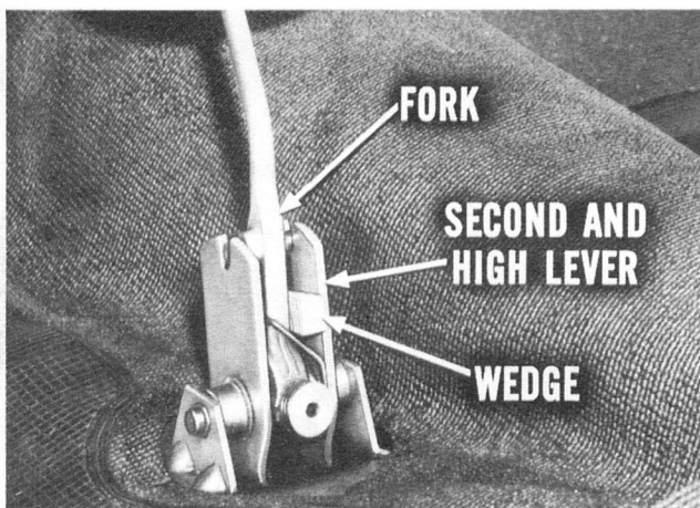
Fig. 13—Wedge keeps crossover pin engaged
