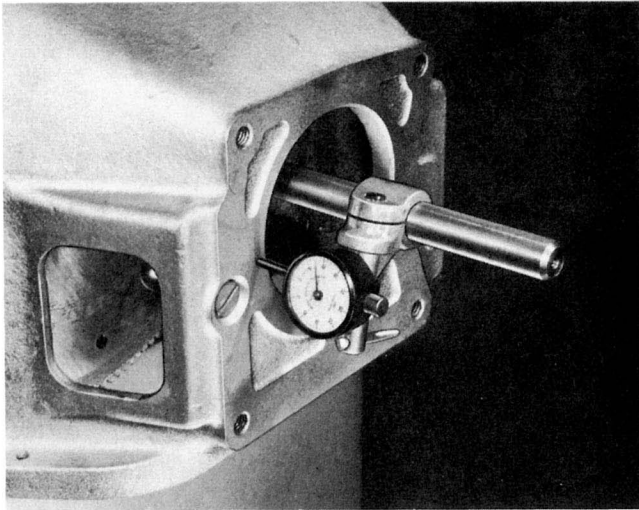
Fig. 21—Measure clutch housing bore and face runout
